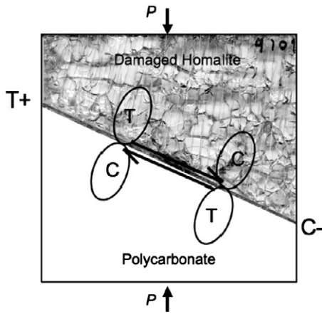
Fig. 5. Anelastic asymmetry results from the positions of the compressive and tensile stress concentration lobes of the two crack tips within the damaged Homalite. In the C direction, the compressive lobe is in the damage while in the T direction the tensile lobe is in the damage. Also shown are the '+' and '-' directions defined by the elastic contrast across the fault. The '+' direction is defined as the direction of motion of the more compliant wall rock (polycarbonate in this case).
