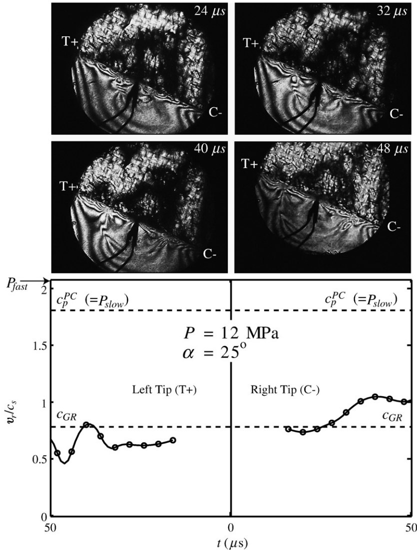
Fig. 6. The same as Fig. 3 except the bilateral shear rupture propagates along a frictional interface separating damaged Homalite above and undamaged polycarbonate below. The rupture tip propagating to the left 'T+' travels at speeds below c_{GR} , the generalized Rayleigh speed. The tip propagating to the right accelerates to speeds in excess of c_{GR} . All velocities are normalized to the shear wave speed in undamaged Homalite.
