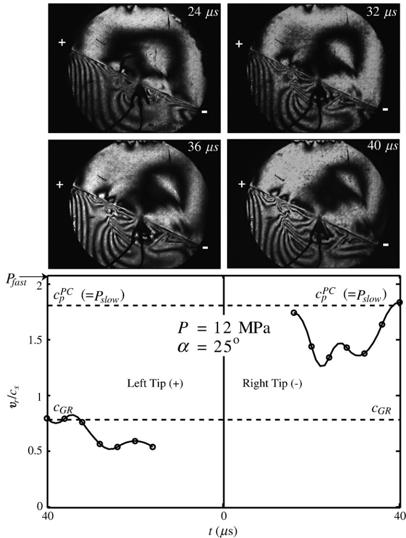
Fig. 3. Snapshots of isochromatic fringe pattern showing rupture contours of maximum shear stress due to a dynamic shear rupture along a frictional interface between an undamaged Homalite plate above and an undamaged polycarbonate plate below. The applied load is P = 12 MPa and the fault angle is \alpha = 25^\circ . Normalized rupture velocity v_r/c_s is plotted as a function of time for the left and right crack tips. The left rupture tip travels in the ‘+’ direction at the generalized Rayleigh speed. The right rupture tip transitions to supershear traveling at P_{slow} , the P-wave speed of the slower material (polycarbonate). Open circles indicate times at which the pictures were taken and the solid curves are the instantaneous rupture velocity found by differentiating cubic spline fits to the measured crack-tip positions as discussed in the text. The normalized P-wave speed in the faster material (Homalite) is 2.08 (the upper boundary of the graph). More fringes appear in the polycarbonate because it has a larger photoelastic constant.
